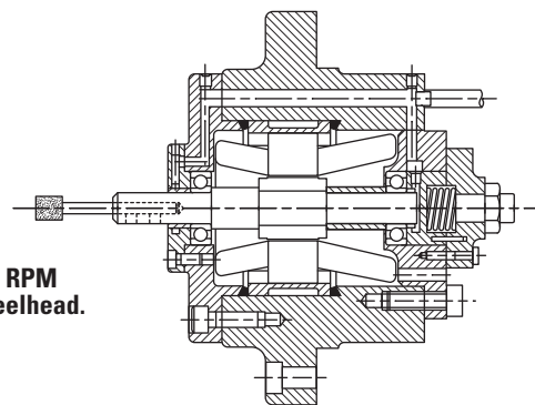
Fig. 113. Single-bar machine.
