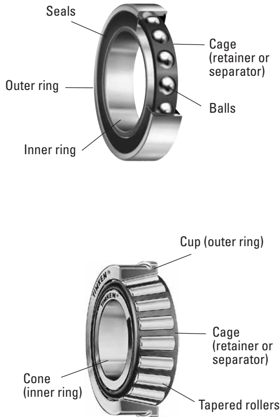
Fig. 2. Bearing components.
