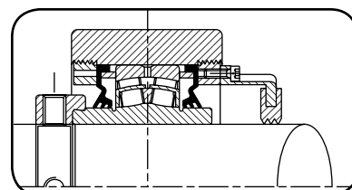
Fig. 29. Open-end urethane cover with DR seal.
