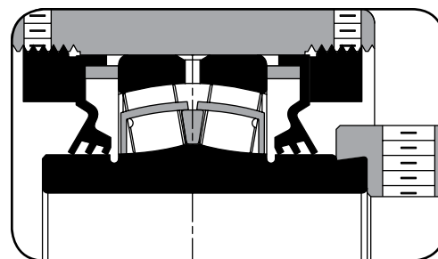
Fig. 25. Triple-lip seals.
