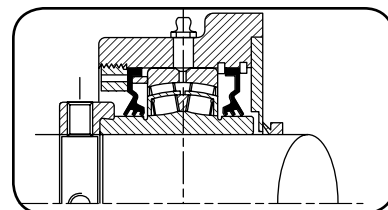
Fig. 32. UFP backing plate with VR seal.
