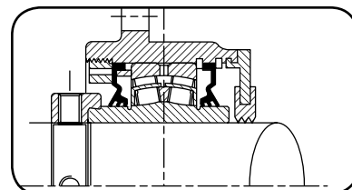
Fig. 31. HSY backing plate with DR seal.
