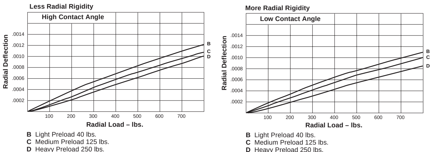
Figure 4-11 – Radial Deflections
