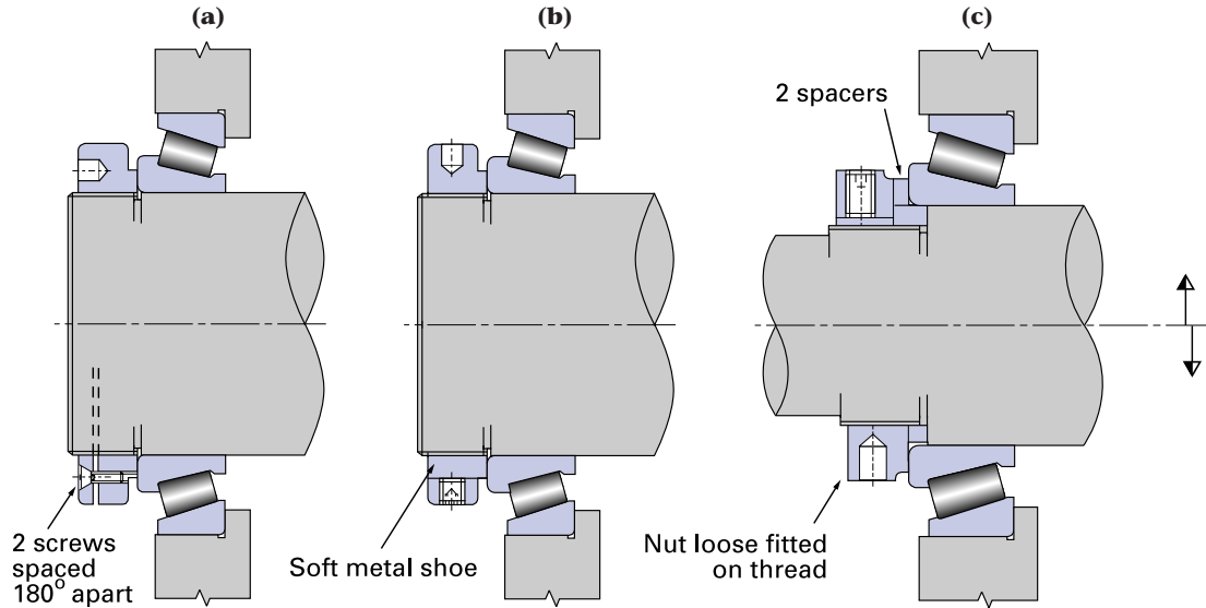
Fig. 4-12 Locking devices
