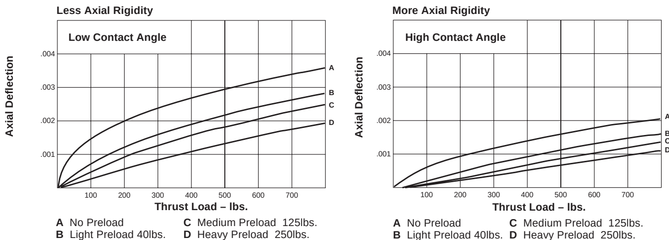
Figure 4-10 – Axial Deflections
