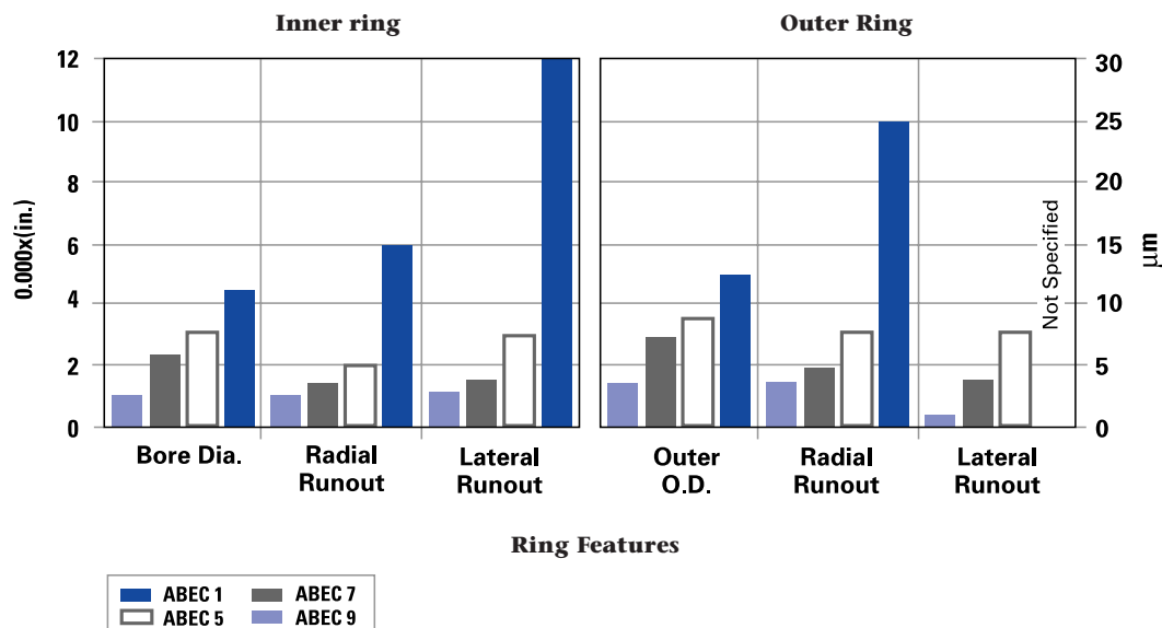
ABEC Tolerances (Light Series, 35mm Bore Type)
