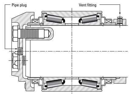
Fig. 42 Mounting Arrangement 3-C
