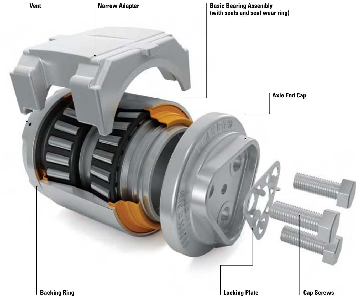
Fig. 1 3D illustration of AP bearing
