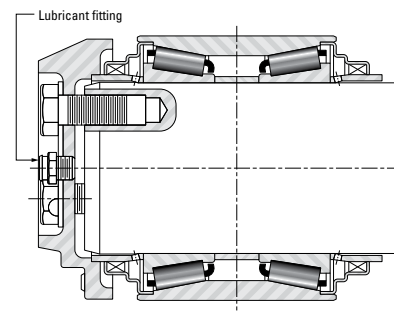
Fig. 39 Mounting Arrangement 3
