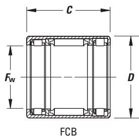
Clutch and Bearing Assemblies
