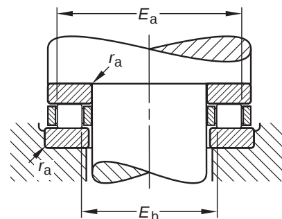
Raceway contact dimensions
