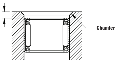
Amount of Recess
