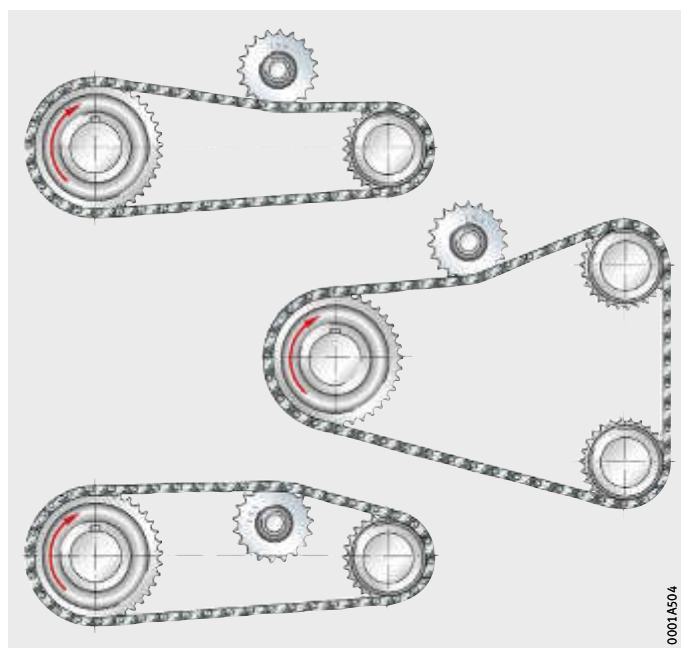
Figure 2 Arrangement on slack side of chain drive
