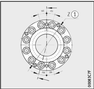
Hole pattern ZARF3080
