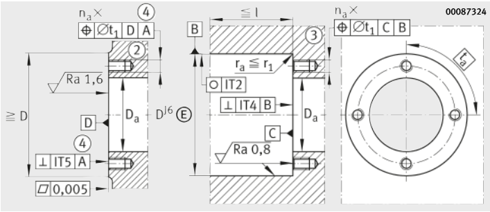
Housing design
