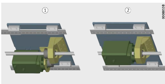
Figure 44 Application examples, rotating screw drive nut
