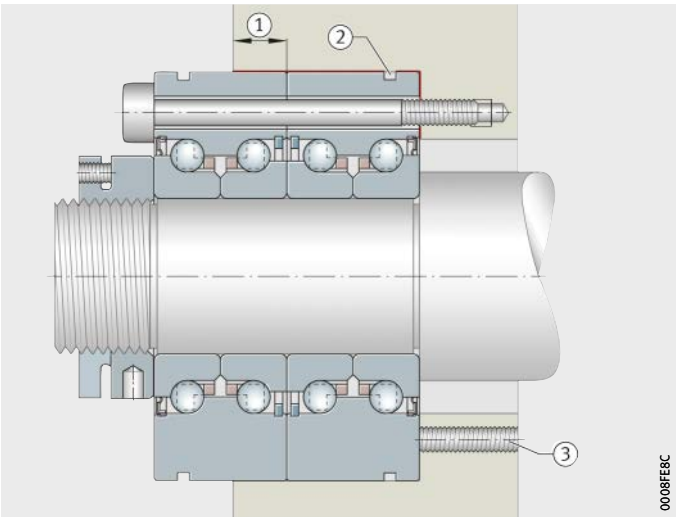
Figure 48 Design example of adjacent construction for ZKLF..-2AP
