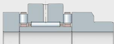
ZARN..-L
