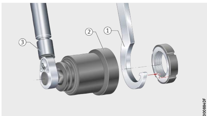
Figure 6 Mounting tools for precision locknuts ZM
