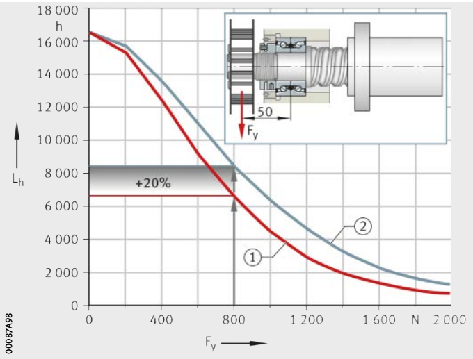
Figure 2 Longer rating life of bearings in O arrangement with additional radial loads
