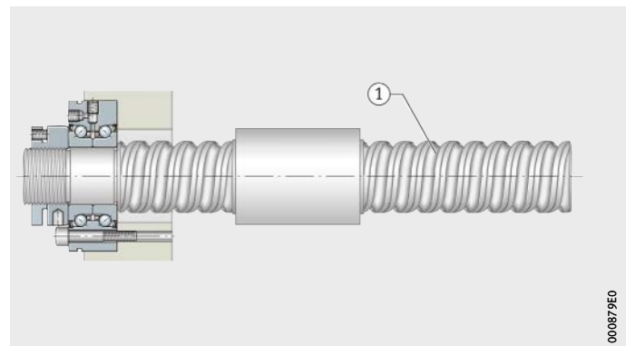
Figure 38 Locating bearing arrangement on one side
