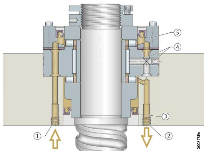
Figure 7 Lubricant feed for vertical mounting position
