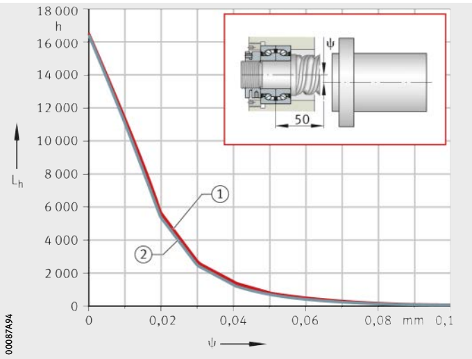
Figure 1 Identical rating life of bearings in X and O arrangement with misalignments between bearing seat and threaded spindle
