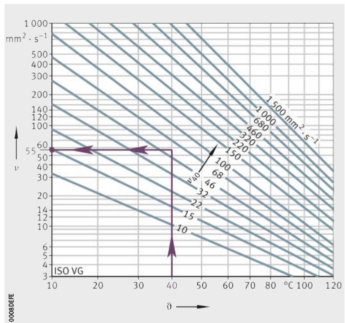
Figure 60 Calculation of operating viscosity \nu at operating temperature \vartheta
