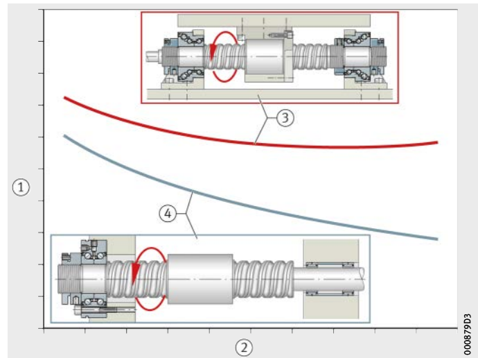
Figure 37 Axial overall rigidity
