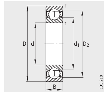
2RSR seal
