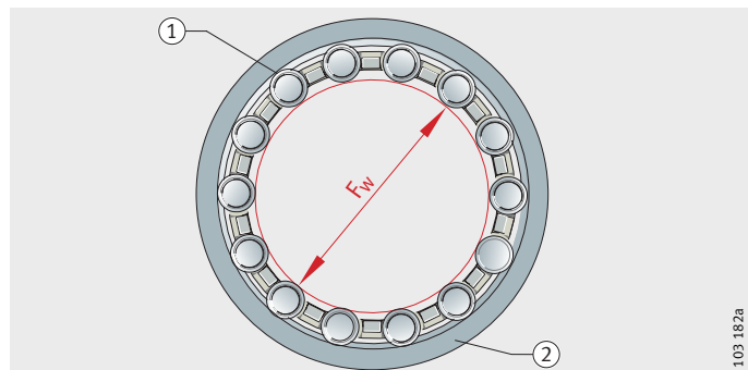
Figure 2 Enveloping circle F_w
