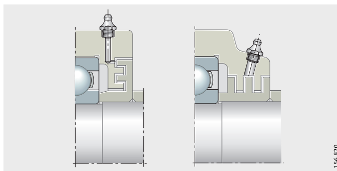
Figure 31 Labyrinth seals
