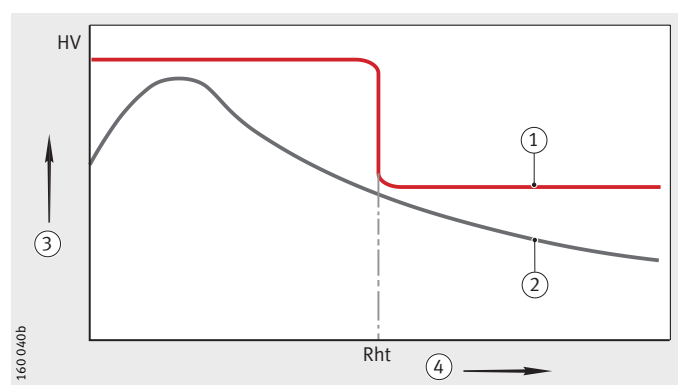
Figure 18 Effective hardening depth Rht
