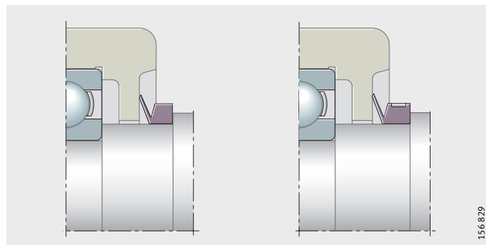
Figure 41 V ring
