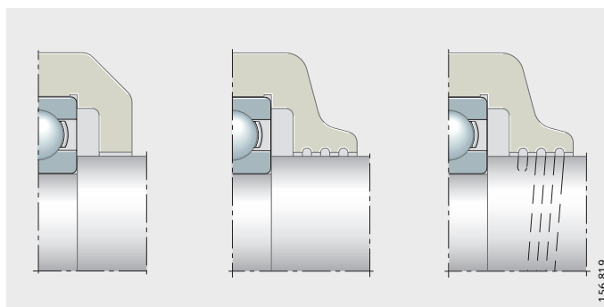
Figure 30 Simple gap seal
