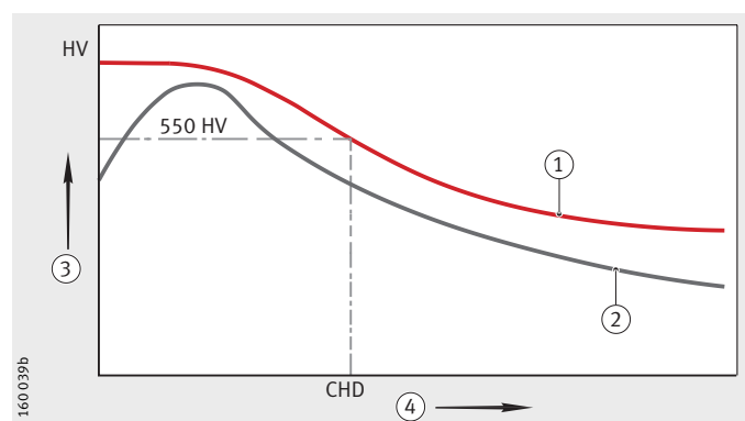
Figure 17 Case hardening depth CHD – hardness curve
