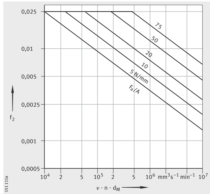
Figure 3 Bearing factor f_2 as a function of operating parameter \nu \cdot n \cdot d_M
