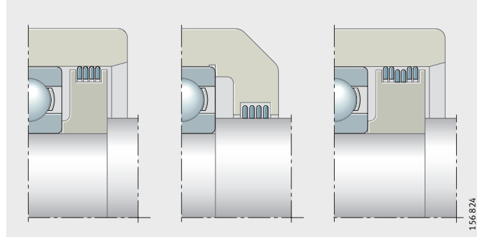
Figure 35 Lamellar rings
