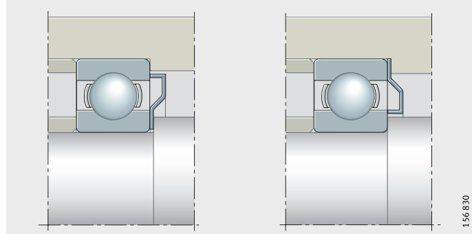
Figure 42 Spring seals
