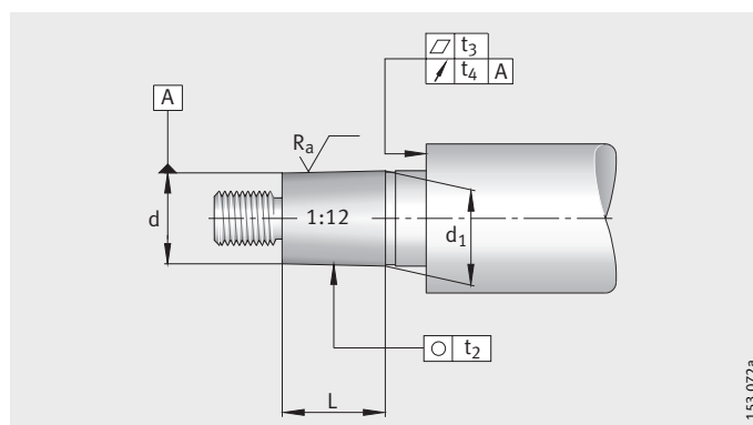
Figure 1 Design of shaft
