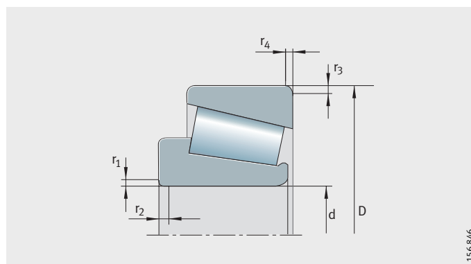
Figure 14 Chamfer dimensions for metric tapered roller bearings
