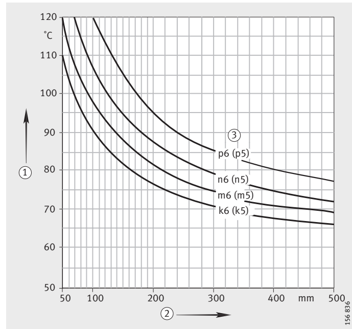
Figure 5 Heating temperature
