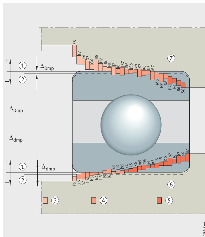
Figure 14 Fits for rolling bearings
