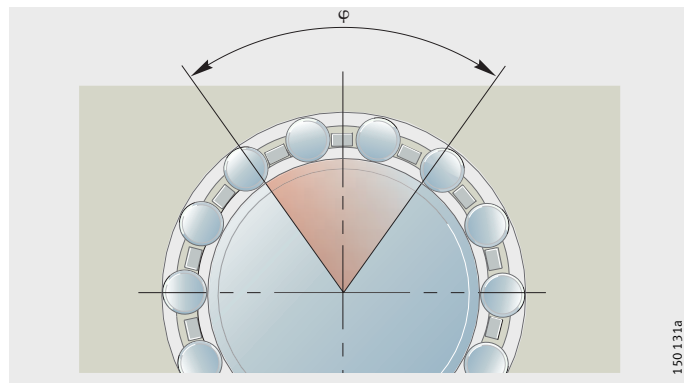
Figure 8 Angle of oscillation \varphi
