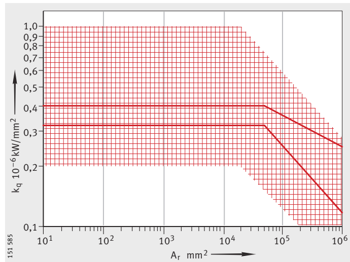
Figure 2 Heat transfer coefficient k_q as a function of the bearing seating surface A_r
