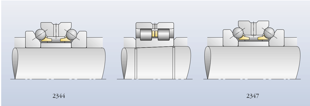
Orientation of double direction angular contact thrust ball bearings of series 2344 and 2347 in relation to double row cylindrical roller bearings
