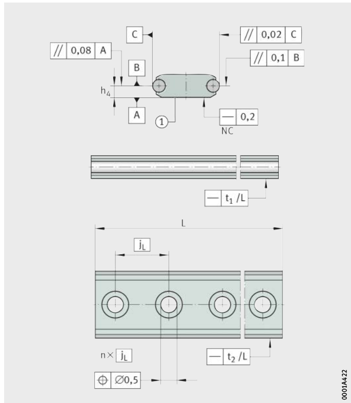
Figure 2 Guideway LFS...-F
