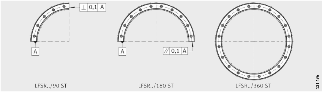
LFSR..-ST
