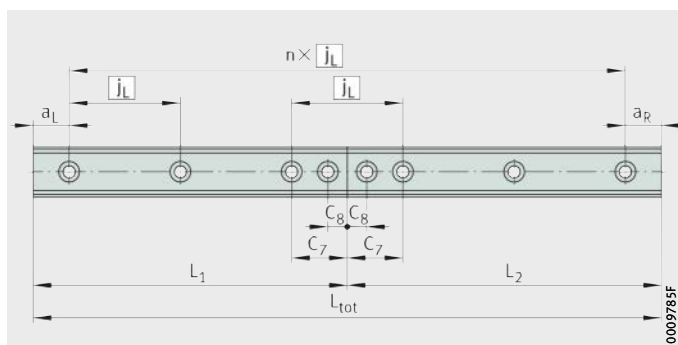
Figure 4 Additional hole
