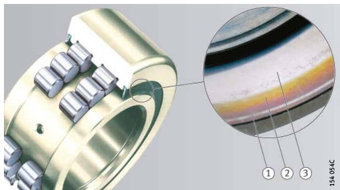
Figure 2 Seal running surface
