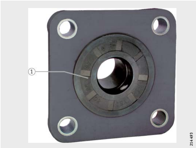
① Back Seal component Figure 2 PCJ with Back Seal component
