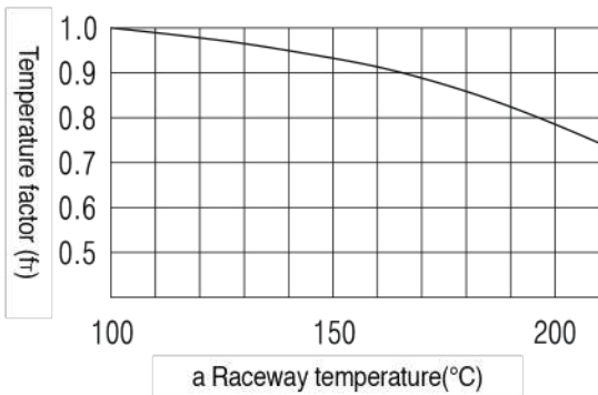
Fig2 Temperature factor(f T )
