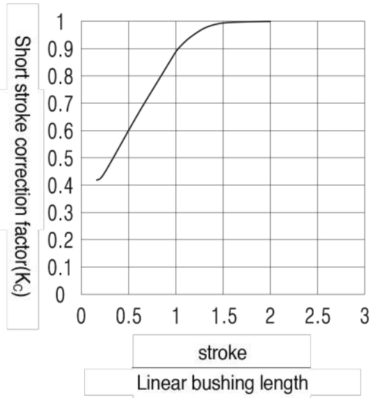
Fig 5. Short stroke correction factor( K_c )
