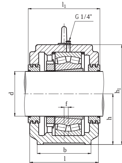
Design B Housing for through shafts
