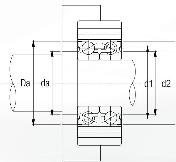
Mounting dimensions
