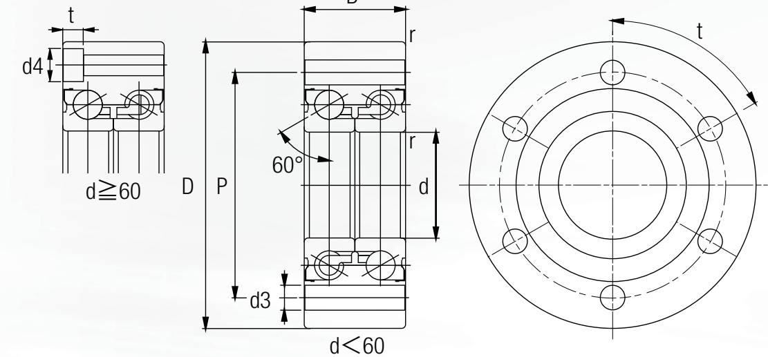
Bearing dimensions
