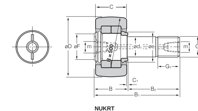
Cam followers stud type truck rollers
