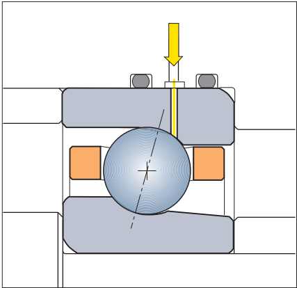
“H1” BEARING
