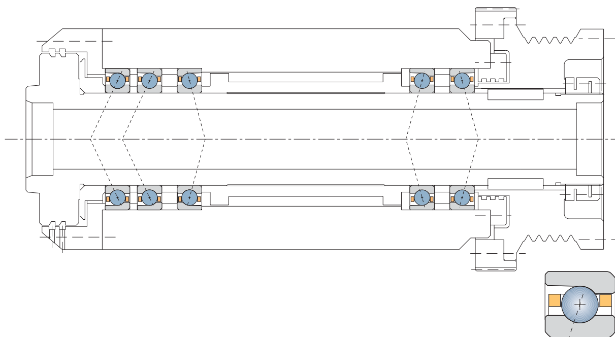
Spindle for a CNC lathe Bearing series EX - Grease lubrication
