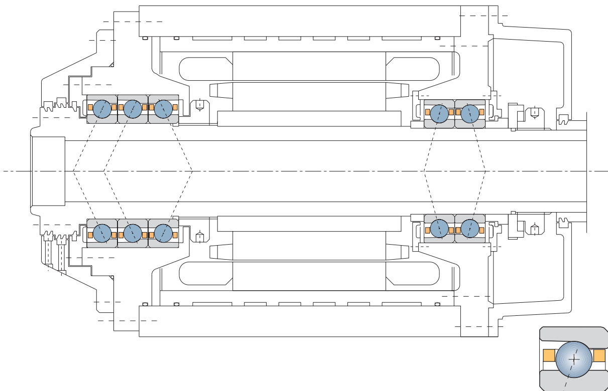
Motorised work head for turning Bearing series SEB - EX - Grease lubrication
