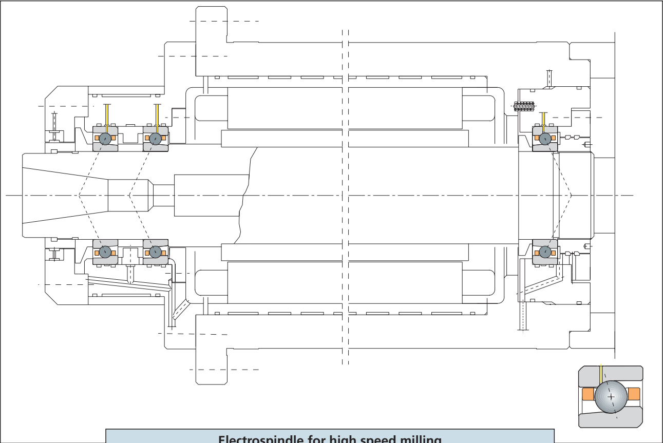
Electrospindle for high speed milling Bearing series VEX/NS/H1 - variable preload Air/oil lubrication throught the outer ring
