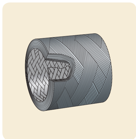
Cross section of SKF filament wound bushing
