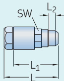
AP 8 and AP 10
