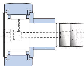
KRE .. PPA ( 22 \leq D \leq 26 \text{ mm} )
