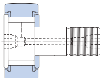
KRV .. PPA ( 22 \leq D \leq 26 \text{ mm} )
