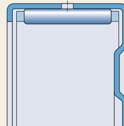
Single row drawn cup needle roller bearing with a lubrication hole in the outer ring
