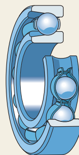
Bearing with filling slots
