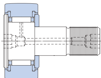
KR .. PPA ( 22 \leq D \leq 26 \text{ mm} )
