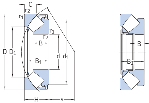
E design
