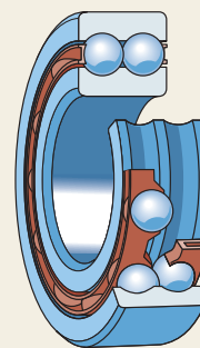
Double row bearing
