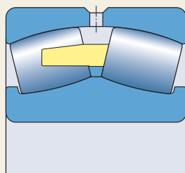
CA design
