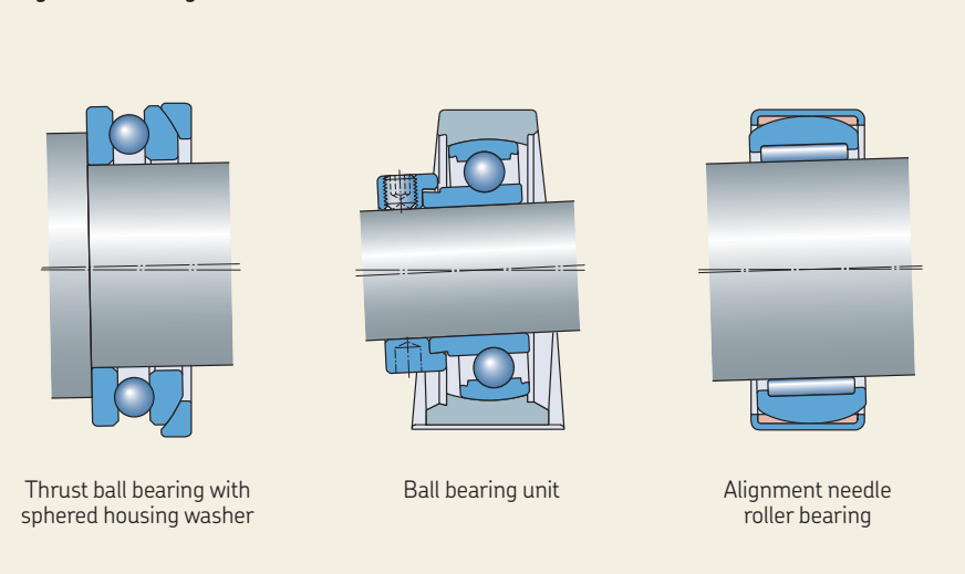
Alignment bearings
