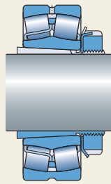
On a plain shaft
