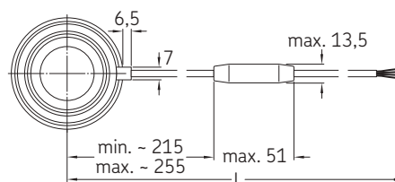
BMB ... 008A (Free cable end) BMO ... 008A (Free cable end)
