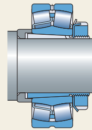
On a stepped shaft
