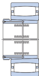
Bearing on an AOH sleeve
