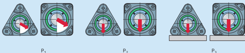
Breaking loads for housings of SKF ConCentra roller bearing units in the FYNT series
