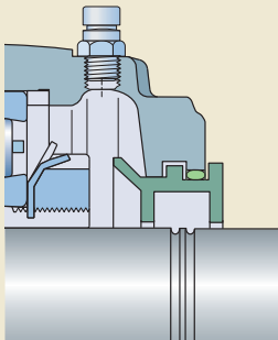
Seal for large axial movements
