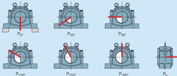
Breaking loads for large SNL plummer block housings made of grey cast iron
