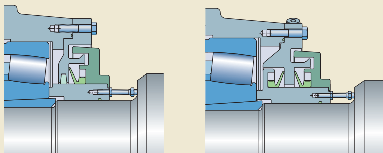
Labyrinth seal with one V-ring seal
