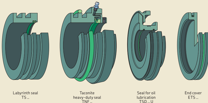
Standard sealing solutions for large SNL plummer block housings
