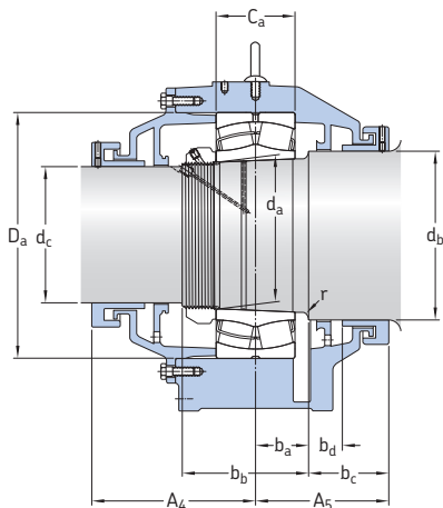
Housing for through shaft (design suffix B)
