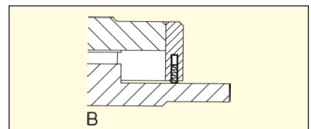
B: End wipers
