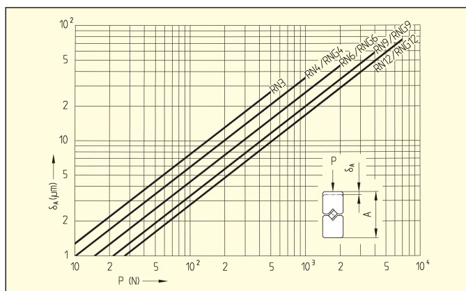
Diagram 2: Elastic deformation of type RNG linear bearings with reference to P per roller
