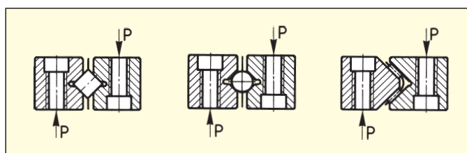
Diagram 4: Elastic deformation of type N/O linear bearings with reference to P for N/O per pair of needles
