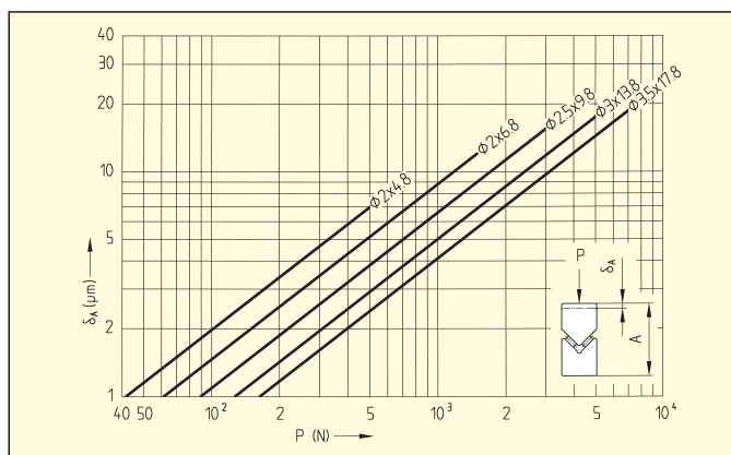
Diagram 4: Elastic deformation of type N/O linear bearings with reference to P for N/O per pair of needles
