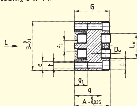
Recirculating Unit NRT
