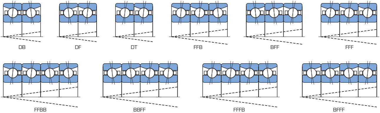
Figure 4.1 Set Combinations and Outer Ring Combination Marks
