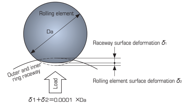
Figure 2.2 Permanent Indentation
