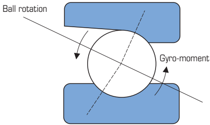
Figure 5.1 Gyro-moment
