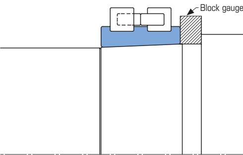
Figure 9.10 Spacer Temporary Width Dimension Measurement
