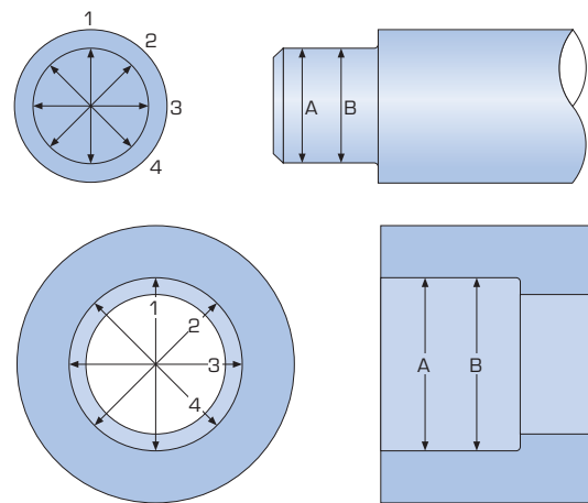
Figure 9.1 Shaft Diameter and Housing Diameter Measurement Locations
