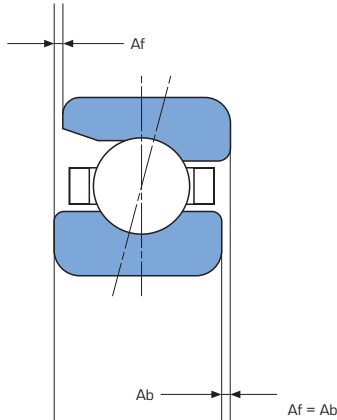
Figure 4.2 Flush Ground Angular Contact Ball Bearing
