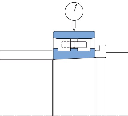
Figure 9.11 Final Assembly Radial Clearance Check
