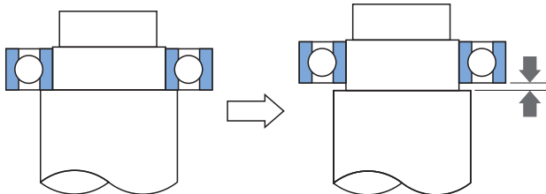
Figure 9.3 Shaft Shoulder Gap After Cooling
