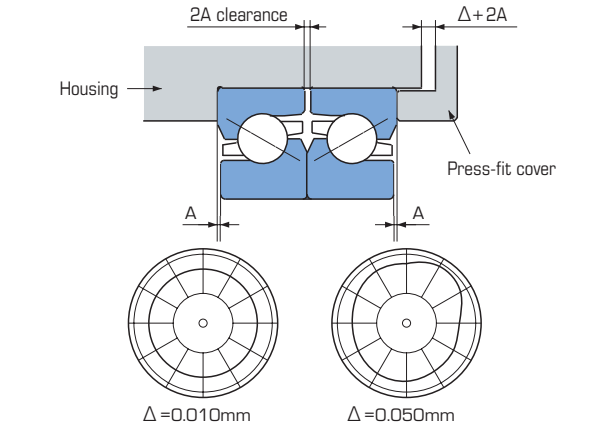
Figure 9.7 Example of Raceway Deflection Depending on Outer Ring Clearance Reduction Gap
