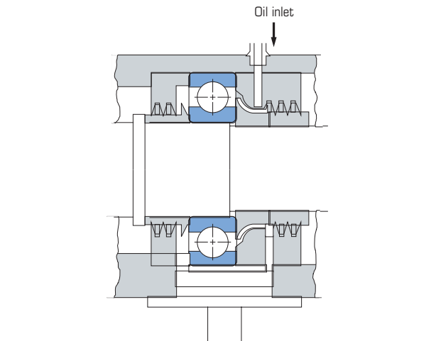
Figure 6.3 Example of Mist Oil Delivery by Slinger
