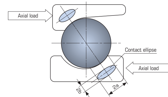
Figure 2.3 Contact Ellipse
