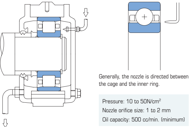
Figure 6.1 Jet Lubrication Example
