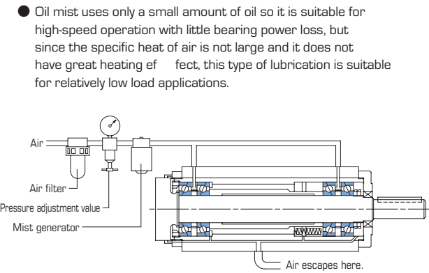
Figure 6.2 Example of Spindle Unit Using Vapor Lubrication
