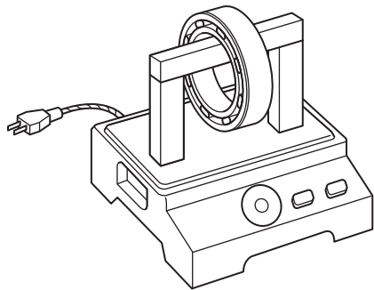
Figure 9.2 Induction Heater
