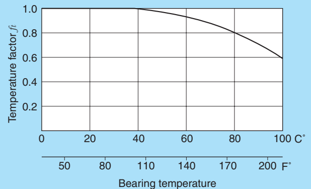
Fig. 1 Temperature factor f_t
