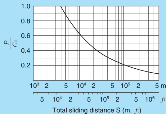
Fig. 3 Load applied to the bearing and the total sliding distance
