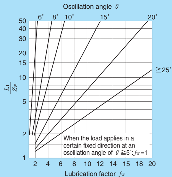
Fig. 6 Lubrication factor f_w
