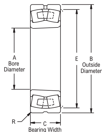
Tapered Bore
