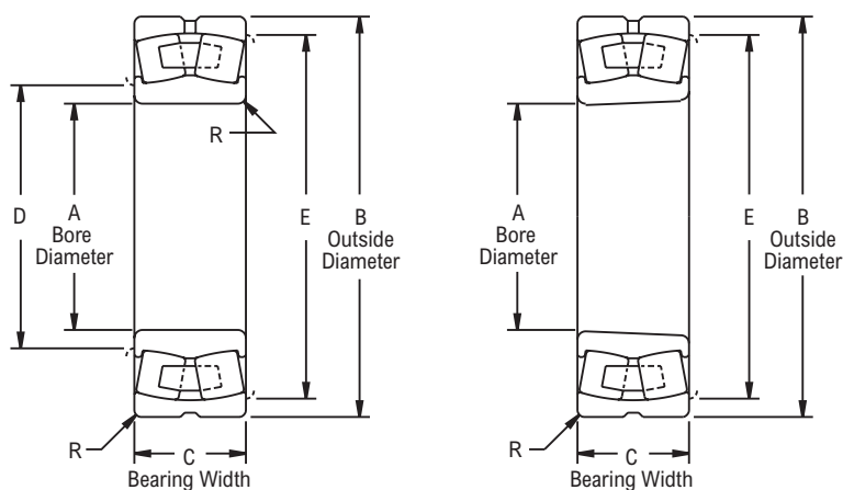
Cylindrical Bore
