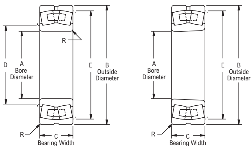
Cylindrical Bore
