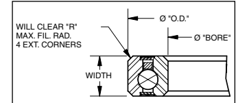
Sealed Bearing
