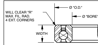
Open Bearing
