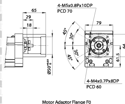
Motor Adaptor Flange FO
