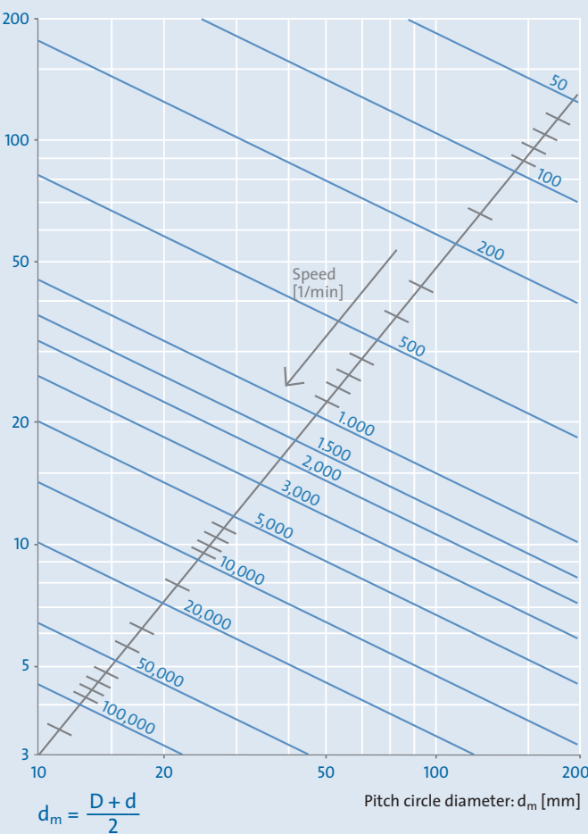
Operating viscosity v_1 [mm²/s]
