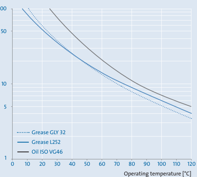
Operating viscosity [mm²/s]
