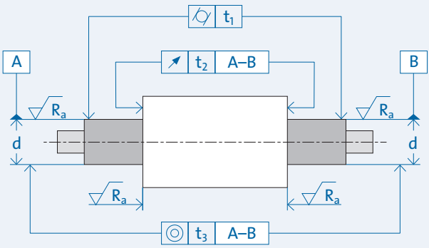
Guidelines for shaft and housing fits / shape and position tolerances (DIN EN ISO 1101)
