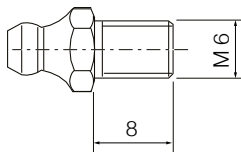
DIN 71412, cone-type nipple for carriage size 25, 30, 35 and 45
