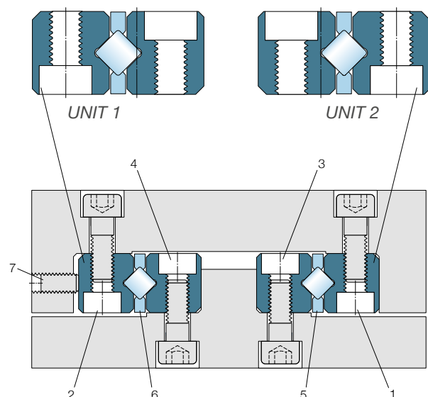
Fig. 8 Mounting sequence
