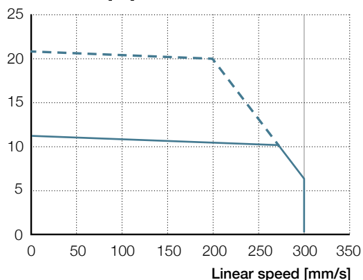
×3W Axial force [kN]
