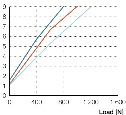
Current-load diagram
