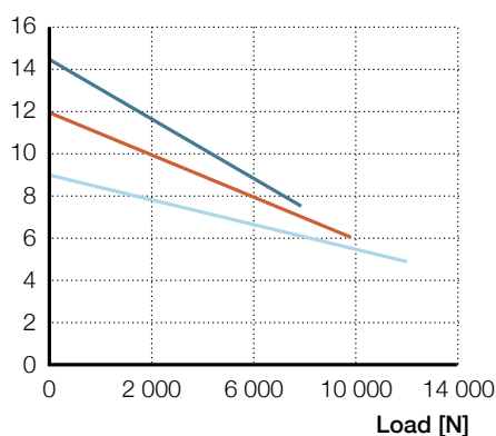
Speed-load diagram
