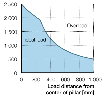
700 mm stroke
