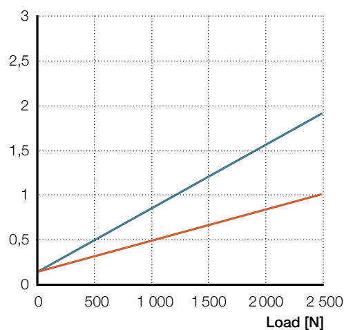
Current-load diagram
