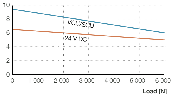
Speed-load diagram
