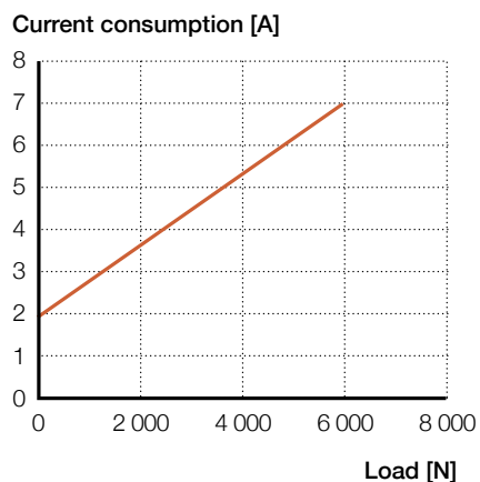
Current-load diagram
