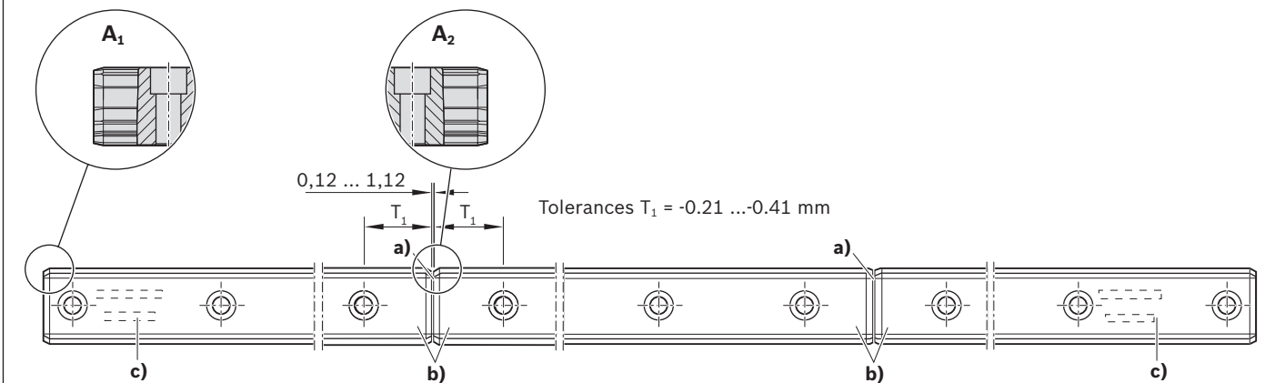
Roller guide rail with universal joint
