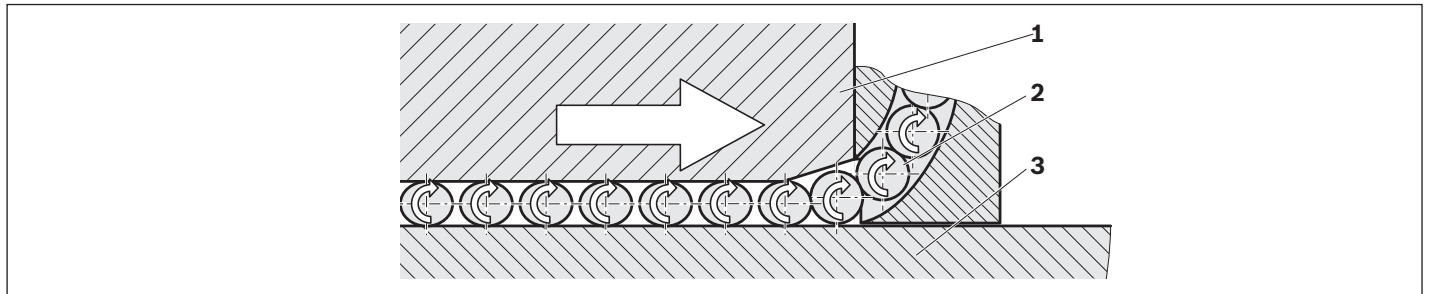
1 Roller runner block 2 Rollers 3 Roller guide rail
